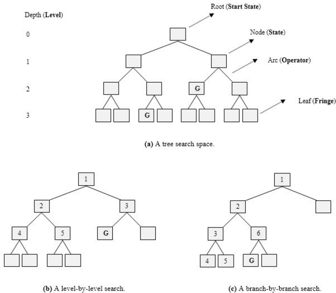
Figure1. The different ways of exhaustive search strategies for a virtual problem.
